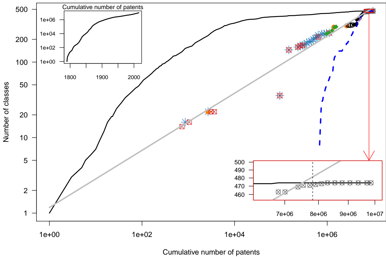
Figure 2: Heaps' law.
